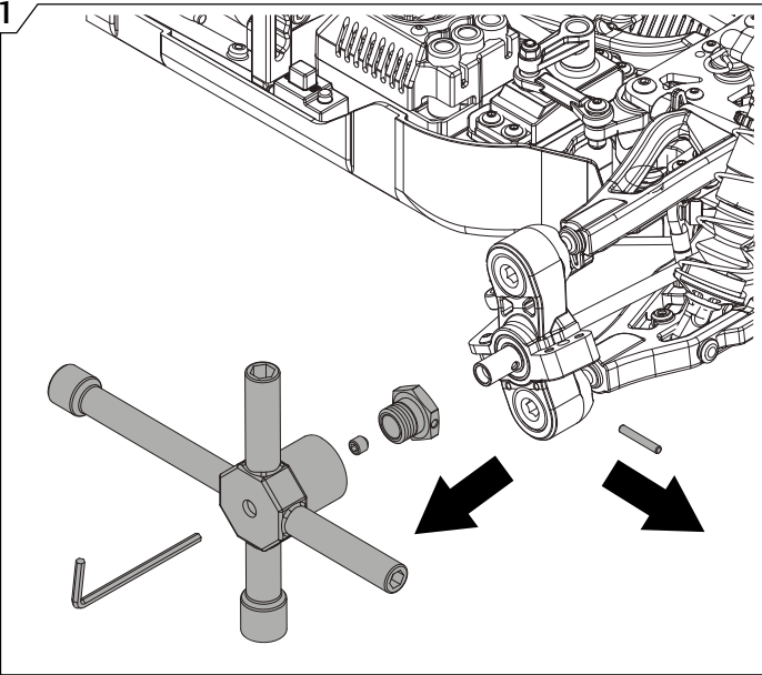
17mm Cross Wrench
